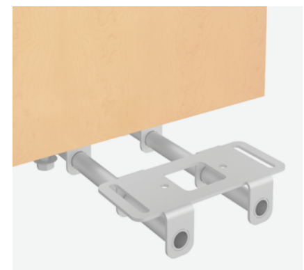
FLOATING TABLE CONNECTION Zola Linking Tables can be easily fastened to Zola Modular seats and benches with the floating table to seat bracket.
